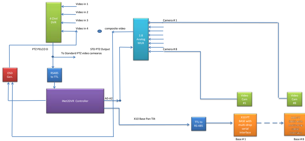
AUX Camera X10 PT base h/w configuration
